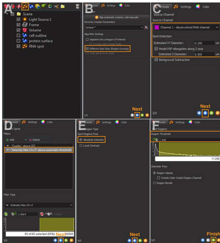
Figure 3. 3D reconstruction of RNA spots. A and B. Create a new spot and select different spot sizes (region growing). C and D. Select source channel and set spot detection. (D) Adjust thresholds and add filters. E and F. Select absolute intensity and adjust region threshold.
