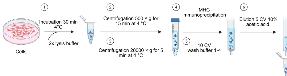
Figure 3. Main steps of the procedure: Generation of cell lysate, immunopurification, and elution of MHC-peptide complexes
