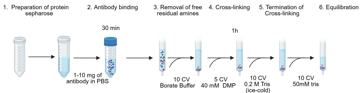
Figure 2. Generation of MHC immunoaffinity column. The first six steps of the procedure are shown and as previously described [13]. CV, column volume; DMP, dimethyl pimelimidate dihydrochloride.
