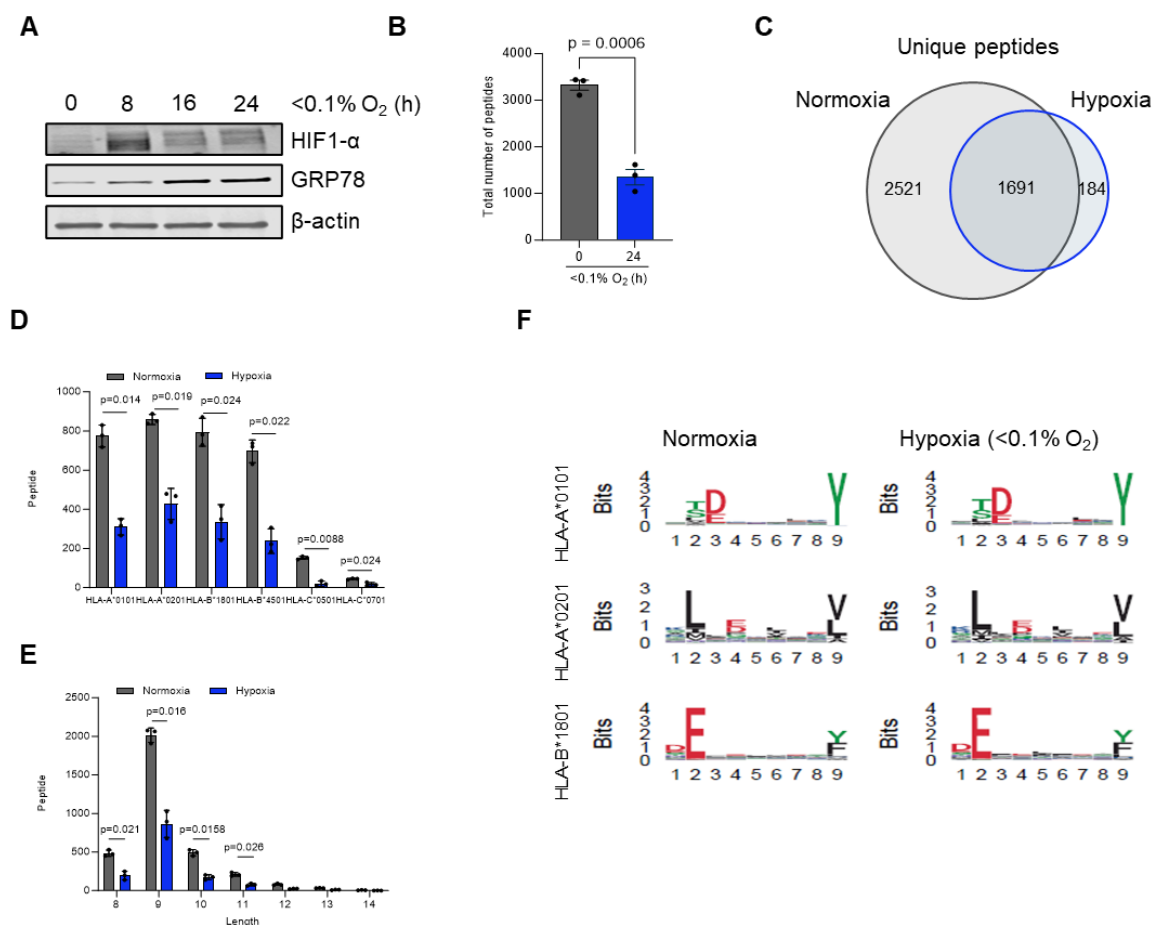
Figure 1. Overview of immunopeptidomics data analysis for cells exposed to normoxia or hypoxia for 24 h. (A) Representative western blot of HT29 cells exposed to hypoxic conditions (<0.1% O 2 ) for the indicated time points. (B) Total number of major histocompatibility complex (MHC) I peptides present on HCT116 cells in normoxia and hypoxia (<0.1% O 2 ). (C) Unique number of MHC I peptides in normoxia vs. hypoxia after 24 h. (D) Allele binding distribution of MHC I peptides. (E) Length frequency distribution of MHC I peptides. (F) Seqlogo comparison of MHC binding motifs in normoxia and hypoxia for three different MHC I subtypes. Peptides were assessed using NetMHCpan 4.1. Data represent mean ± SEM from three biological replicates. Statistical significance was determined using an unpaired Student's t-test. Adapted from Estephan et al. [28].
