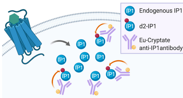
Figure 2. IP-One assay principle. Endogenous IP1 produced after 7TMR activation enter into competition with the exogenous d2-labeled IP1 for binding to the exogenous Eu-cryptate anti-IP1 antibody. When d2-IP1 is bound to the Eu-cryptate anti-IP1 antibody, the close proximity of the two fluorescent dyes allows for energy transfer during the readout (represented by the orange arrow). The more IP1 is produced by 7TMR activation, the less d2-IP1 is bound to the Eu-cryptate anti-IP1 antibody and the less energy transfer can be recorded during readout.
