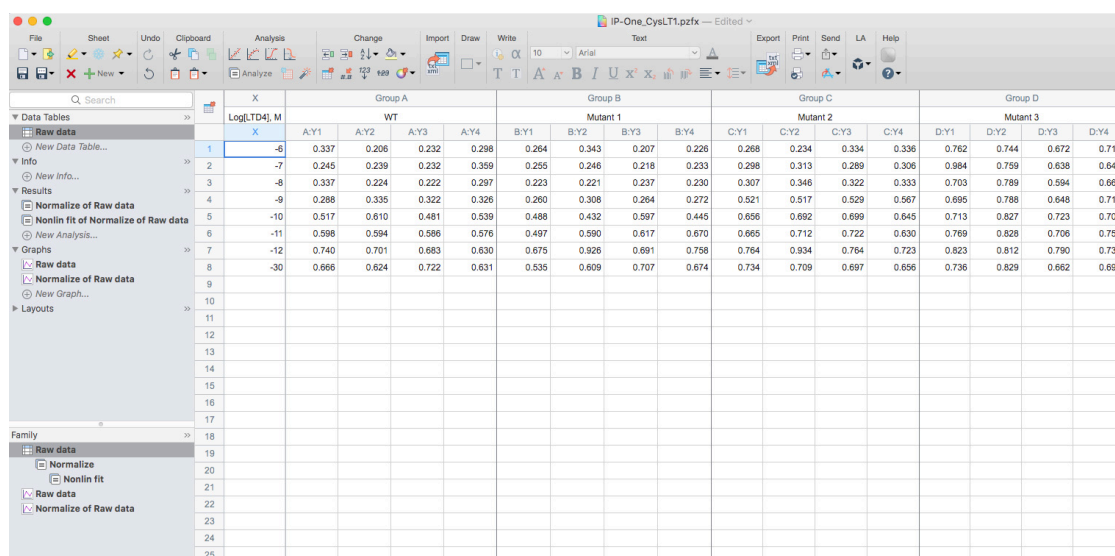
Figure 4. Screenshot example of the raw data of IP1 production for the wild type and mutants of the human CysLT1 receptor
