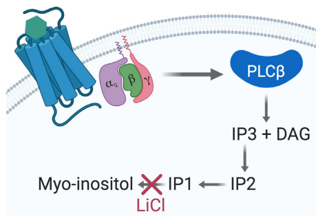
Figure 1. The G_{\alpha q} signaling pathway. Upon agonist binding at a given G_{\alpha q} -coupled 7TMR, the \alpha subunit dissociates from the \beta\gamma dimer and activates the PLC \beta , thus initiating the cleavage of PIP2 into IP3 and DAG. IP3 is then degraded into IP2, IP1, and myo-inositol. Accumulation of IP1 is achieved by using a stimulation buffer containing LiCl to inhibit IP1 degradation into myo-inositol and further recycling.
